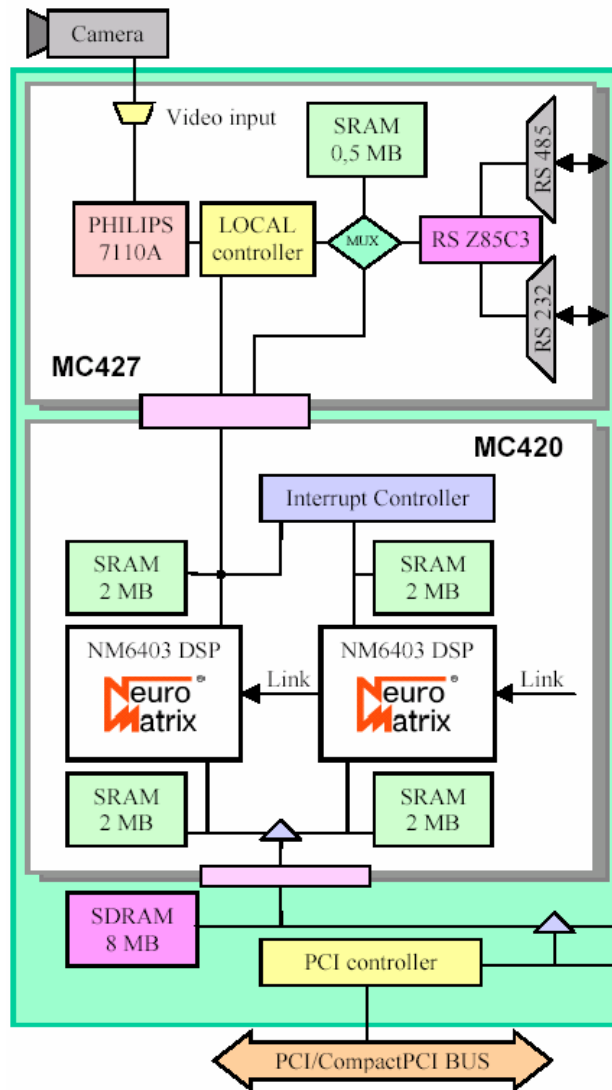
Figure 3: NM6403 based DSP board, from [5]
