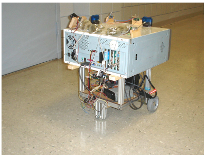
Figure 2c: Riscbot Top view (Back).
