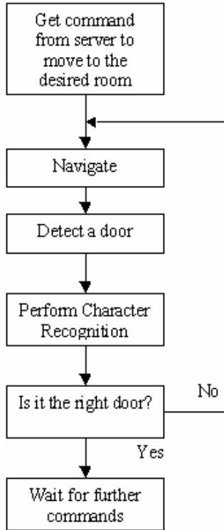
Figure 4: Navigation module.
