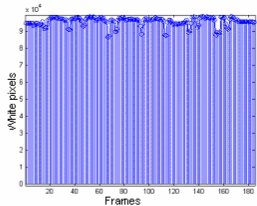
Figure 15: White Pixels (Edges) Vs Frames.
